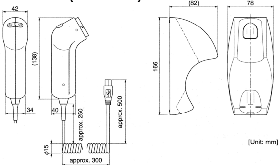
i-Scope Main Body
